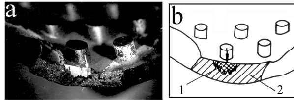
Fig. 9 Photo and diagram of blade fracture along the crack
