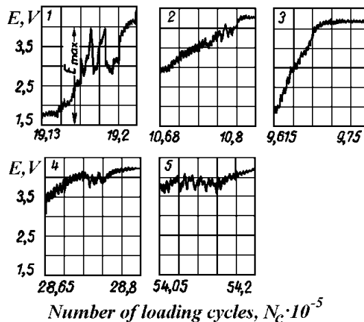
Fig. 2 Acoustograms of AE energy change during cyclic loading of solid blades with the use of E-criterion
