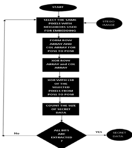
Fig. 8. Data Extracting Process
