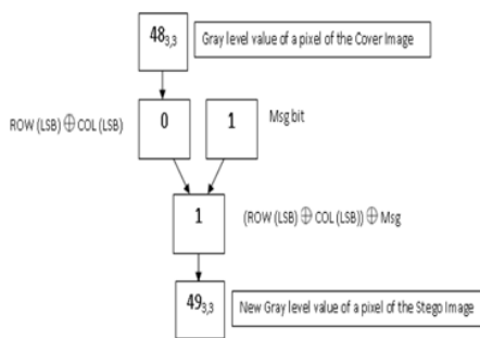
Fig. 7. A snapshot of data embedding process
