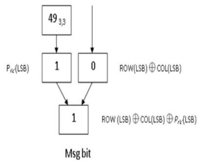
Fig. 9. A snapshot of data extracting process
