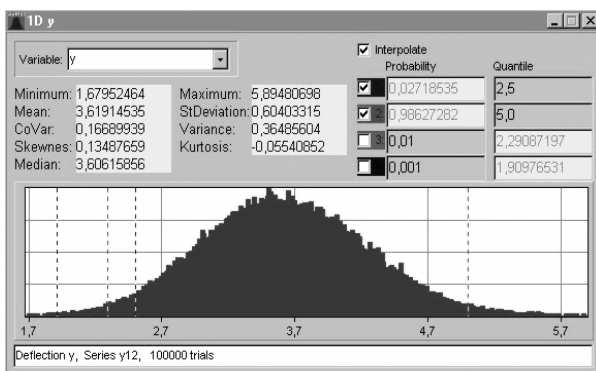
Fig. 3 Screen of the Monte Carlo simulation program Ant-Hill [8]
