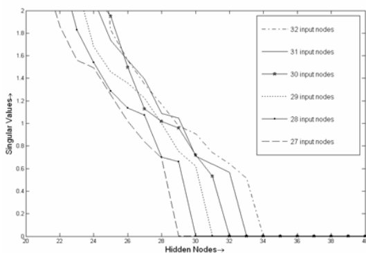
Fig. 9 Singular values of matrix D for different numbers of hidden nodes
