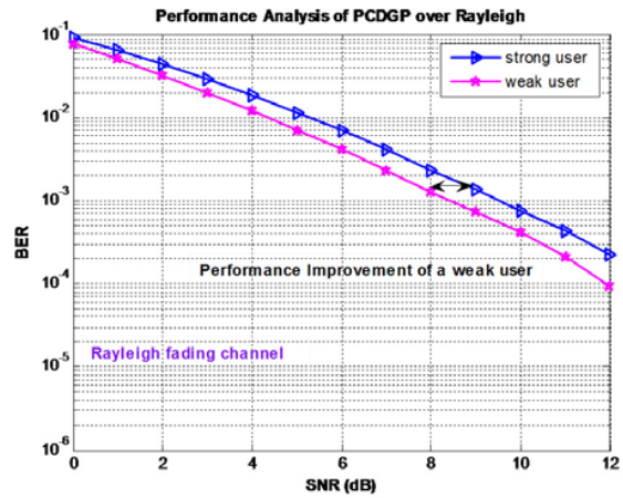
Fig. 2. Simulation results for the PCDGP system for both users over Rayleigh fading channel
