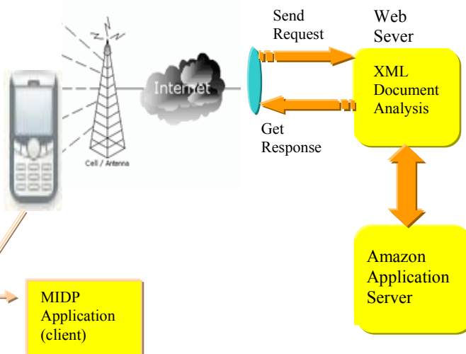
Fig. 2 A detailed description of eCoMobile information retrieval process
